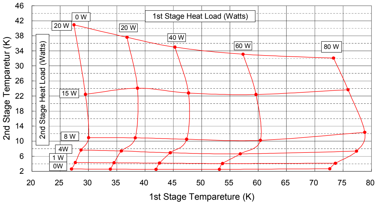
RDK-408D2 Typical Load Map (50Hz)
