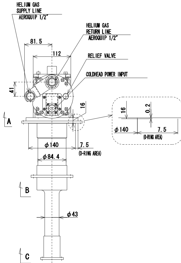
COLD HEAD UNIT
